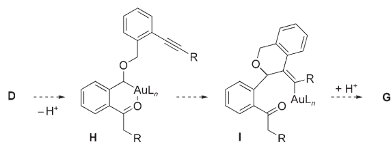
Scheme 6. Conceivable alternative route from D to G .
