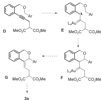
Scheme 5. Conceivable transformation of D to 3g .
