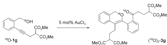
Scheme 3. Intramolecular migration of the oxygen atom of the benzylic alcohol.
