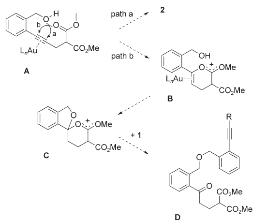
Scheme 4. Proposed mechanism for the formation of the ether bridge between the two substrate units and the intramolecular oxygen transfer.
