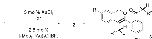
Scheme 2. An unprecedented dimerization was observed with 1g–1k .
