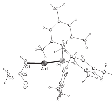
Figure 1. Solid-state structure of [(Mes 3 P)AuCH 2 COCH 3 ].
