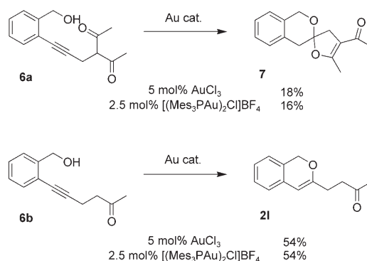
Scheme 7. Products obtained when there are keto groups in the side chain.
